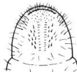
Oriental beetle
