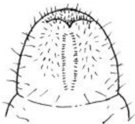
May-June beetle
