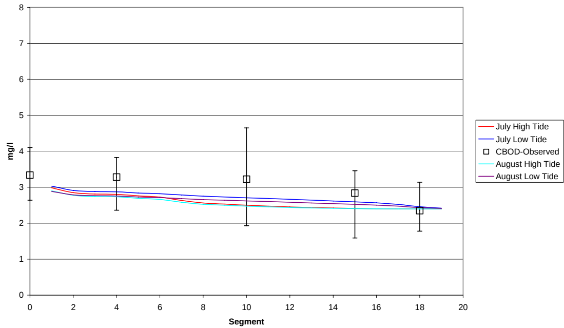
CBOD Model vs. Observed
