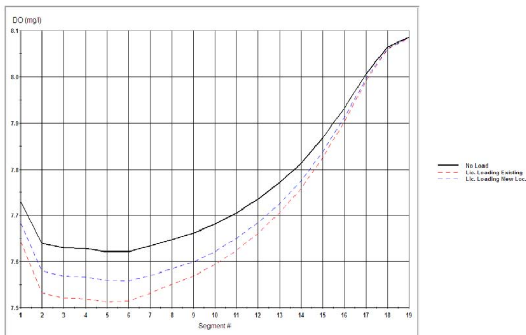
Figure 6: Minimum DO, Predictive Model Run Comparison Critical Conditions
