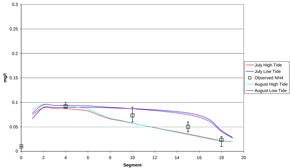
NH4 Model vs. Observed
