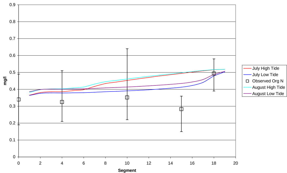
Organic N Model vs. Observed
