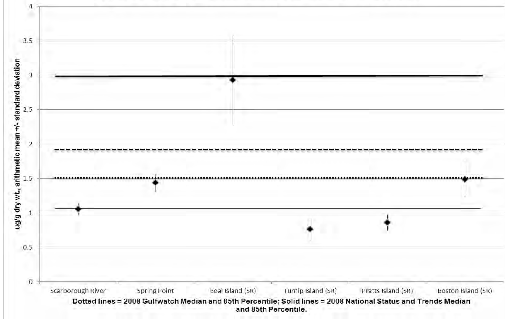
Figure 1.3.1.1.4.1: Chromium in 2012 SWAT Blue Mussels
