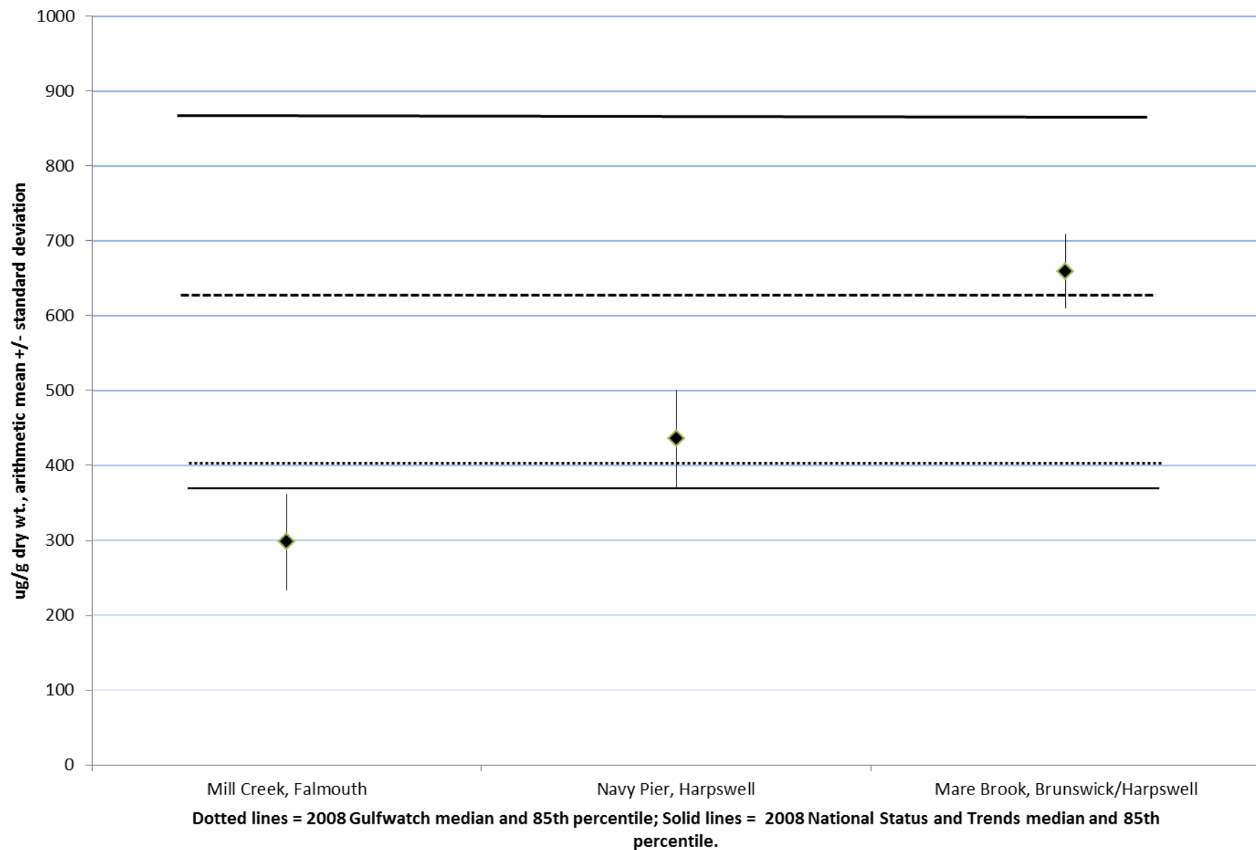
Figure 1.3.1.1.6.1: Iron in 2014 SWAT Blue Mussels
