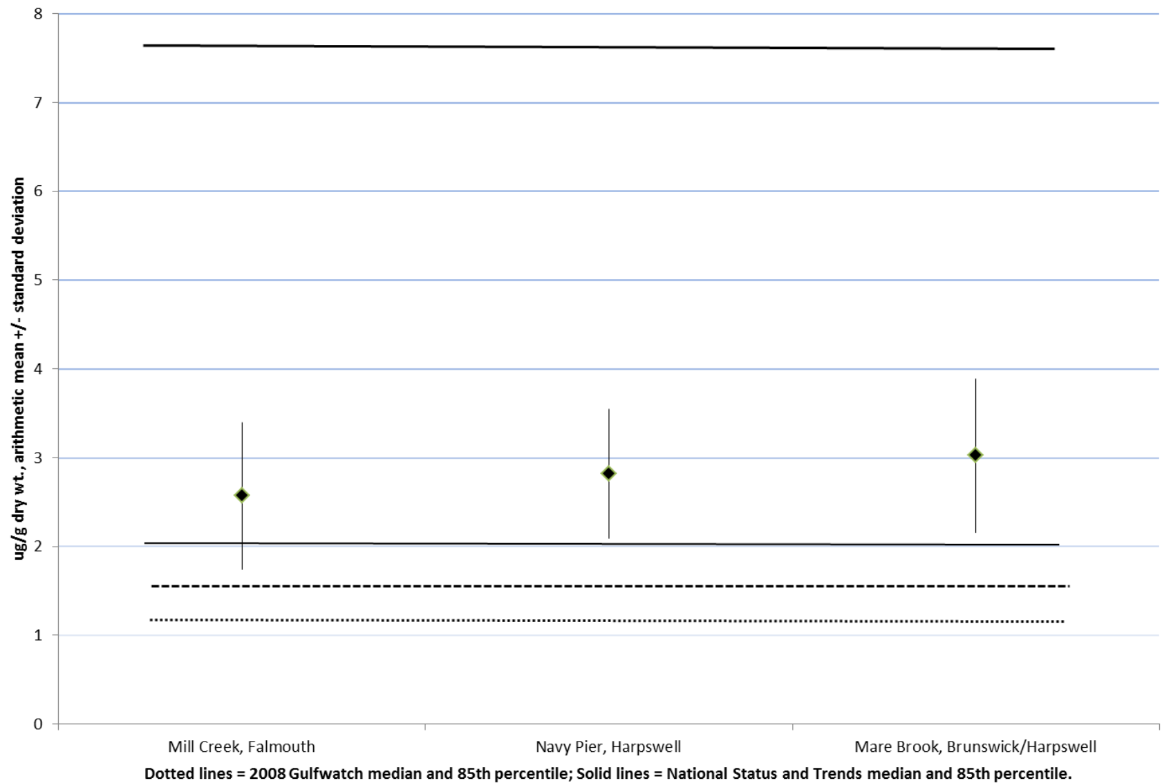
Figure 1.3.1.1.7.1: Nickel in 2014 SWAT Blue Mussels
