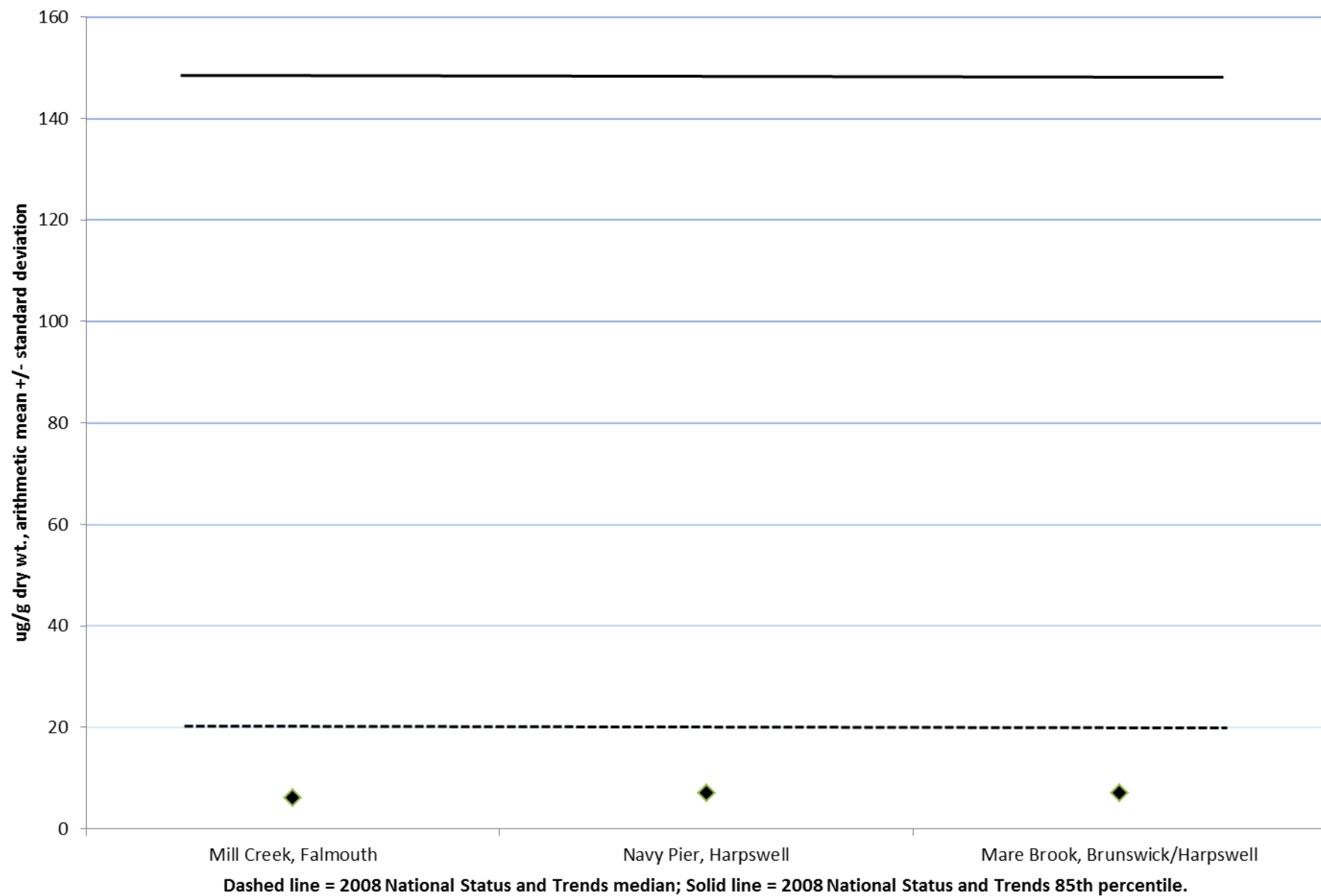
Figure 1.3.1.1.5.2: Copper in 2014 SWAT Blue Mussels
