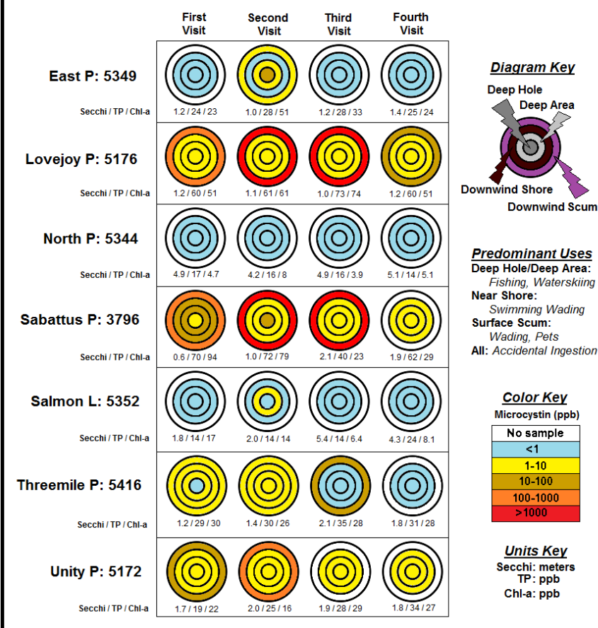
Figure 2.1.3. Time Series Concentrations of microcystin in seven Maine lakes. Lakes were visited 4 times with approximately 2 weeks between visits beginning in late August 2014. Samples were obtained from 3-4 locations on the lake represented by concentric circles. Secchi Transparency depth, Total Phosphorus and Chlorophyll_a concentrations from the Deep Hole are included below each sampling event.
