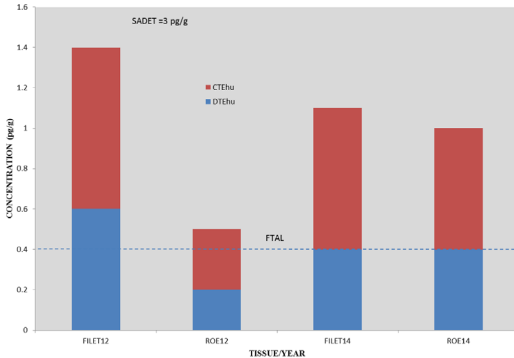
Figure 3.2.1. Dioxin (DTEhu) and coplanar PCB (CTEhu) toxic equivalents (upper 95th confidence limit) in American shad (AMS) filet and roe from Waterville on the Kennebec River (KWV) 2012 and 2014
