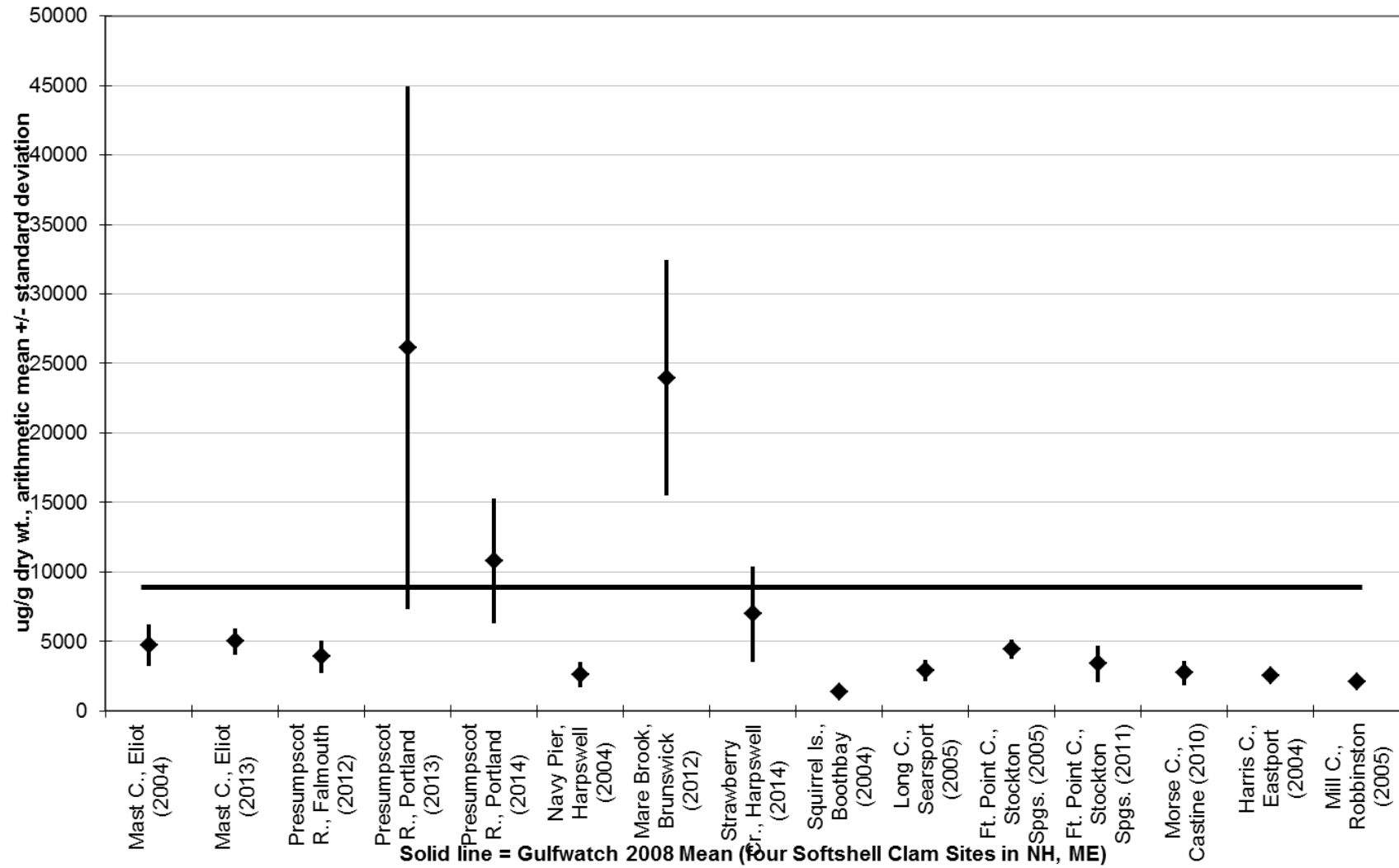
Figure 1.3.1.2.6.1: Iron in SWAT Softshell Clams
