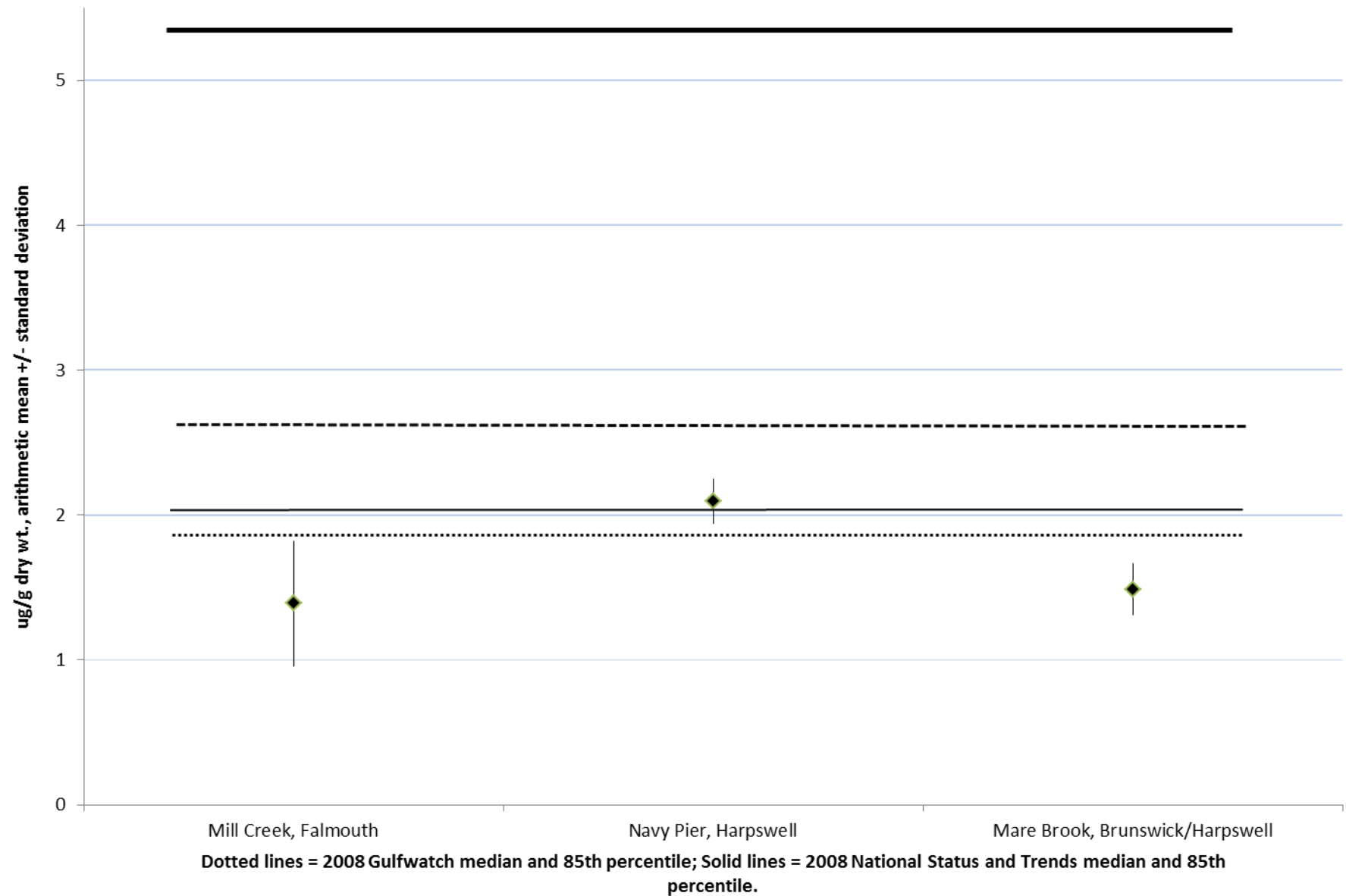
Figure 1.3.1.1.3.1: Cadmium in 2014 SWAT Blue Mussels
