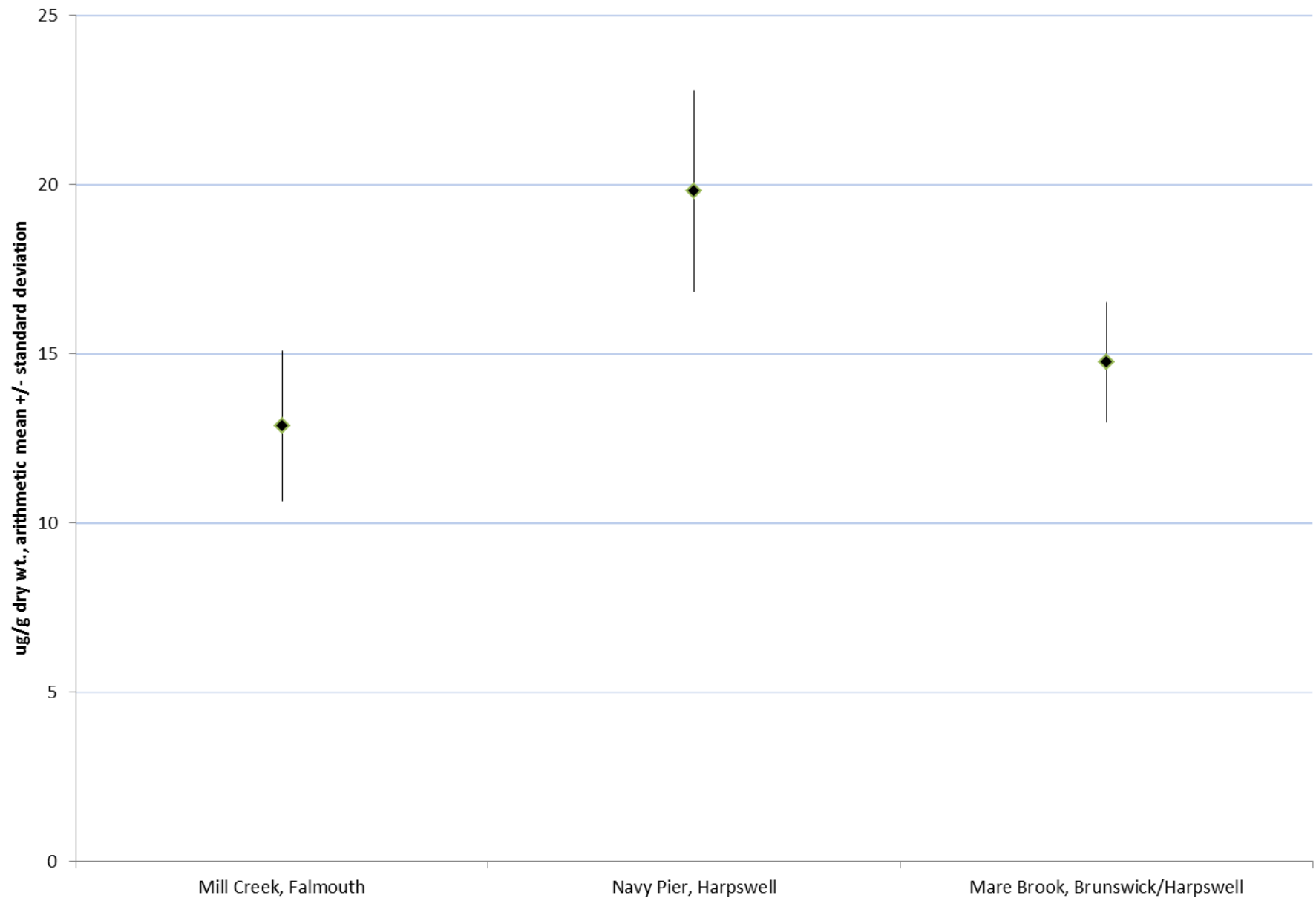
Figure 1.3.1.1.2.1: Arsenic in 2014 SWAT Blue Mussels
