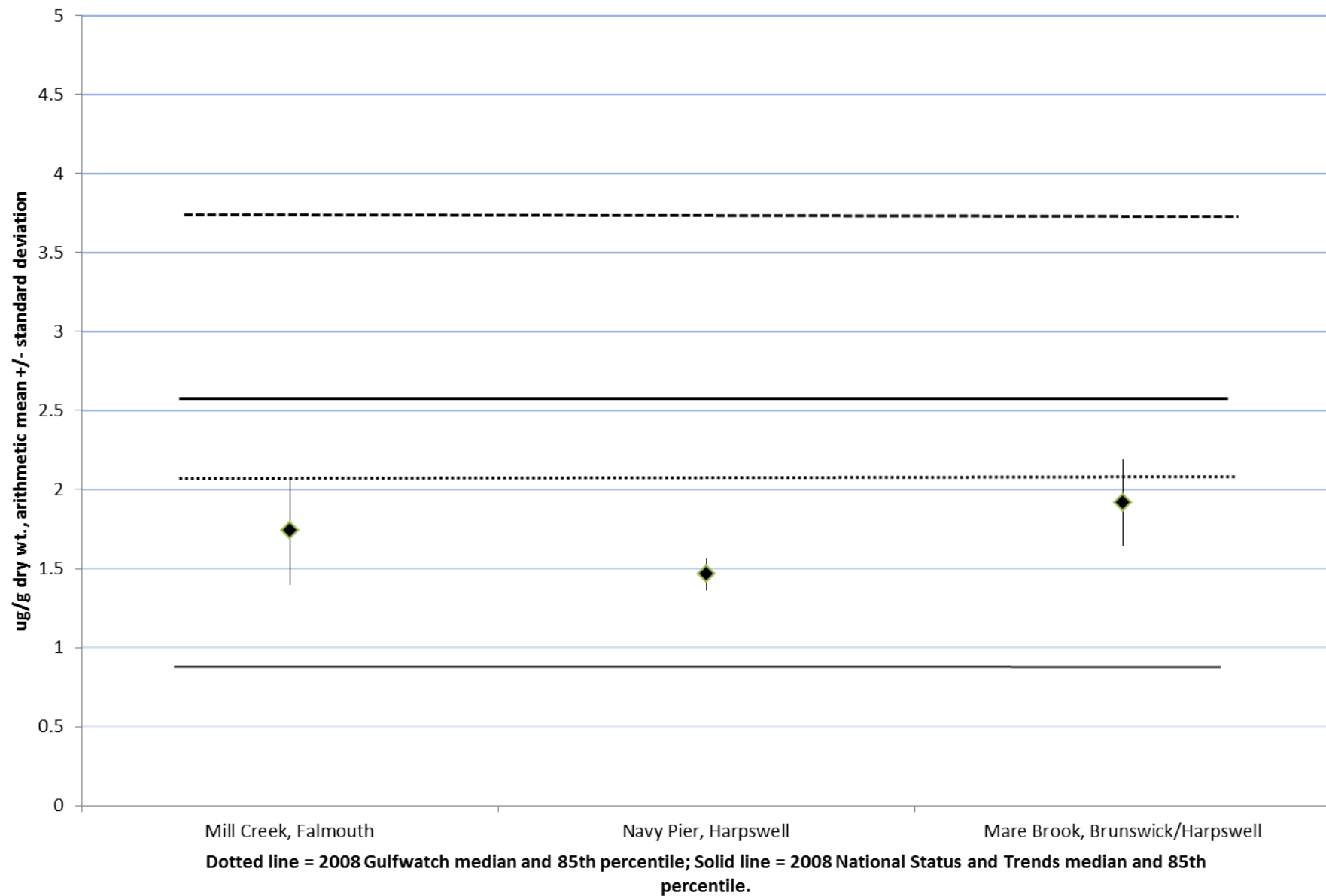
Figure 1.3.1.1.8.1: Lead in 2014 SWAT Blue Mussels
