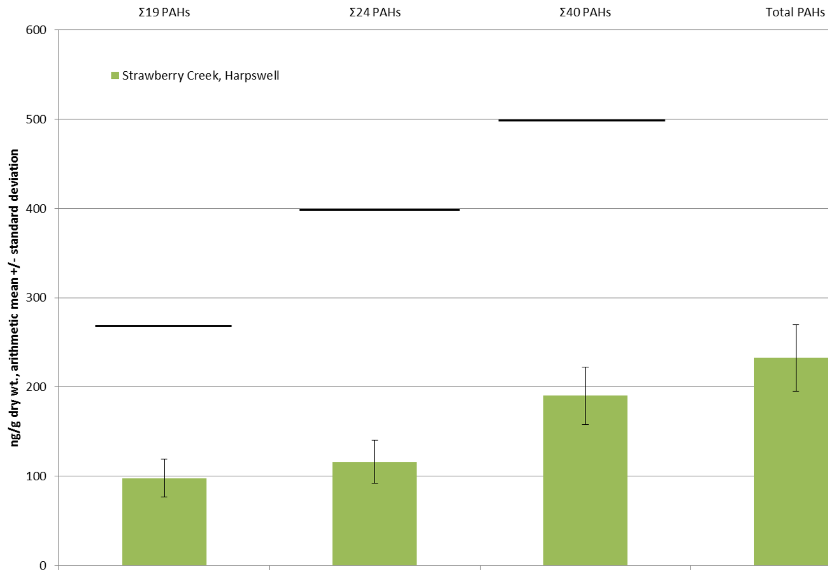
Figure 1.3.2.2.1: PAHs in Softshell Clams
