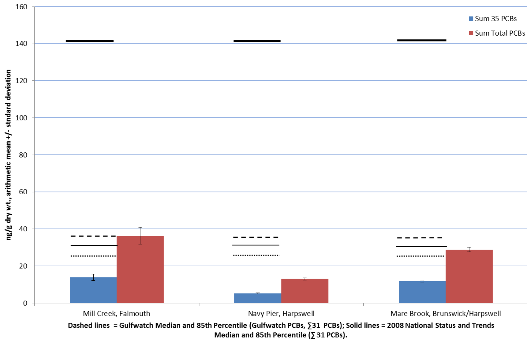
Figure 1.3.3.1.1.: SWAT PCBs ( \Sigma 35 PCBs) and Total PCBs in 2014 SWAT Blue Mussels
