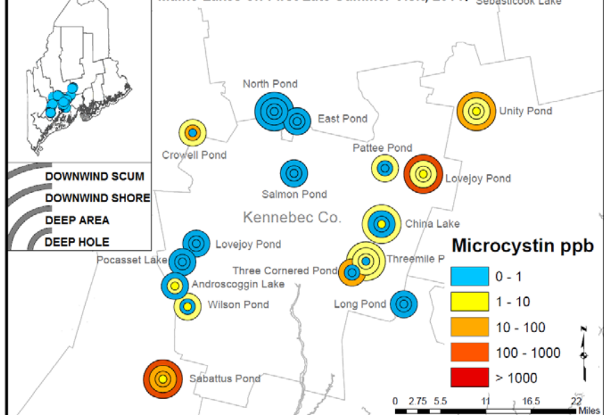
Figure 2.1.2. Microcystin LR Results by Sampling Station in 17 Central Maine Lakes on First Late Summer Visit, 2014.
