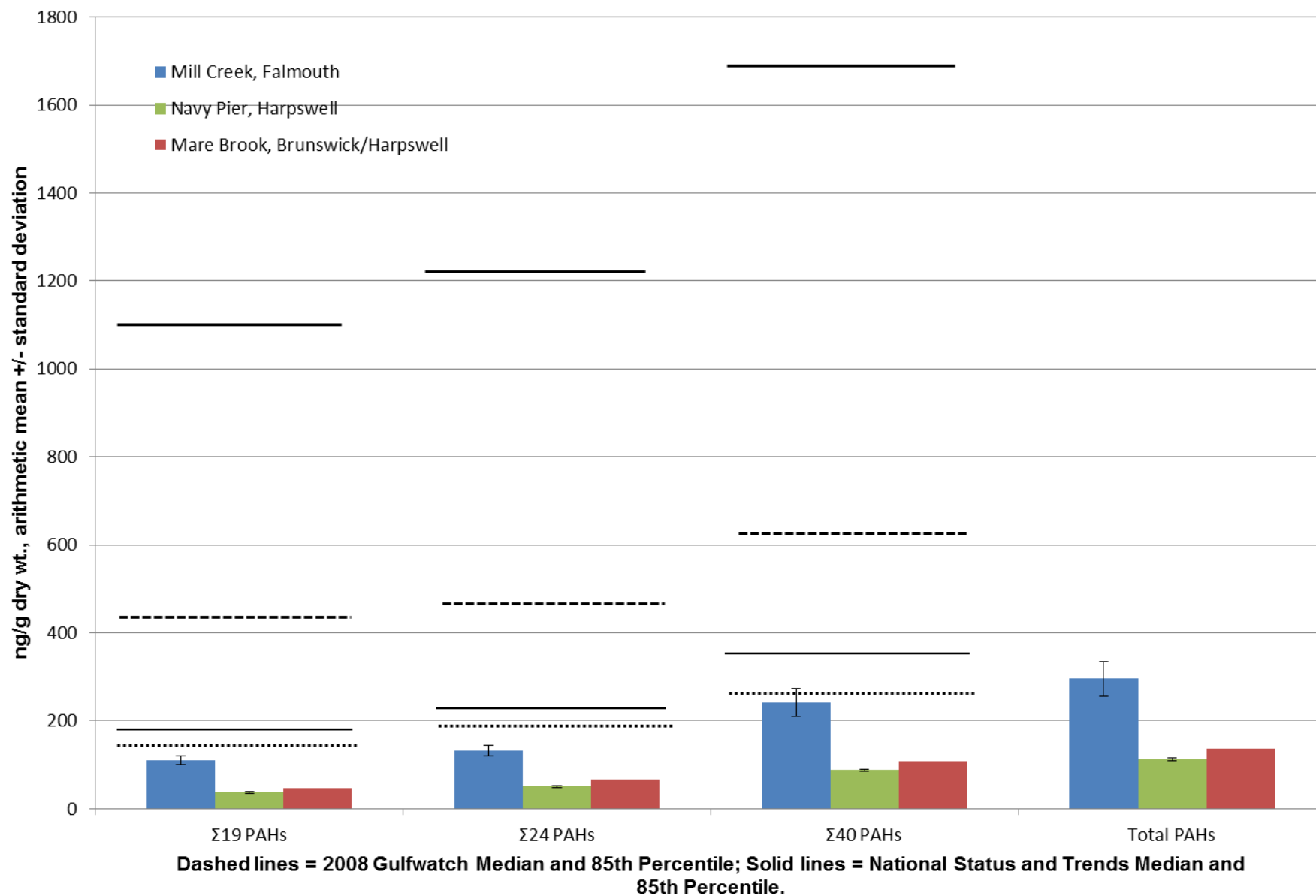
Figure 1.3.2.1.1: PAHs in Blue Mussels
