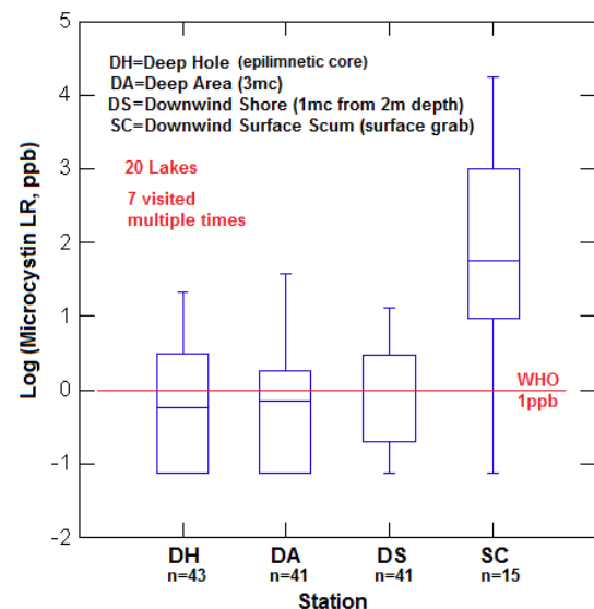
Figure 2.1.1. Distribution of Microcystin LR Concentration by Sampling Station in 20 Maine Lakes, late summer 2014.
