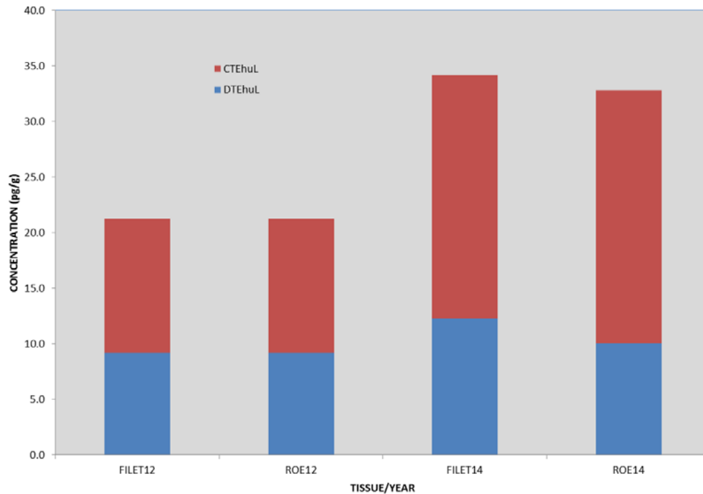
Figure 3.2.2. Lipid normalized Dioxin (DTEhuL) and coplanar PCB (CTEhuL) toxic equivalents (upper 95th confidence limit) in American shad (AMS) filet and roe from Waterville on the Kennebec River (KWV) 2012 and 2014
