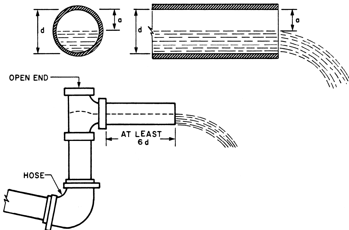
Figure 1: California Pipe Flow Method (USEPA, August 1973)
