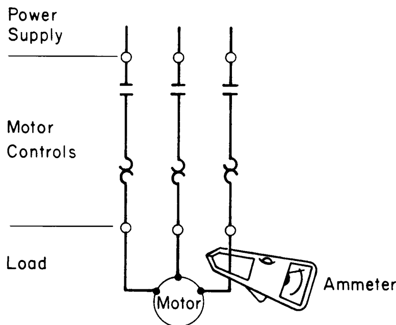
Figure 18: Checking 3-Phase Motor Amperage (Adapted from Flygt)
