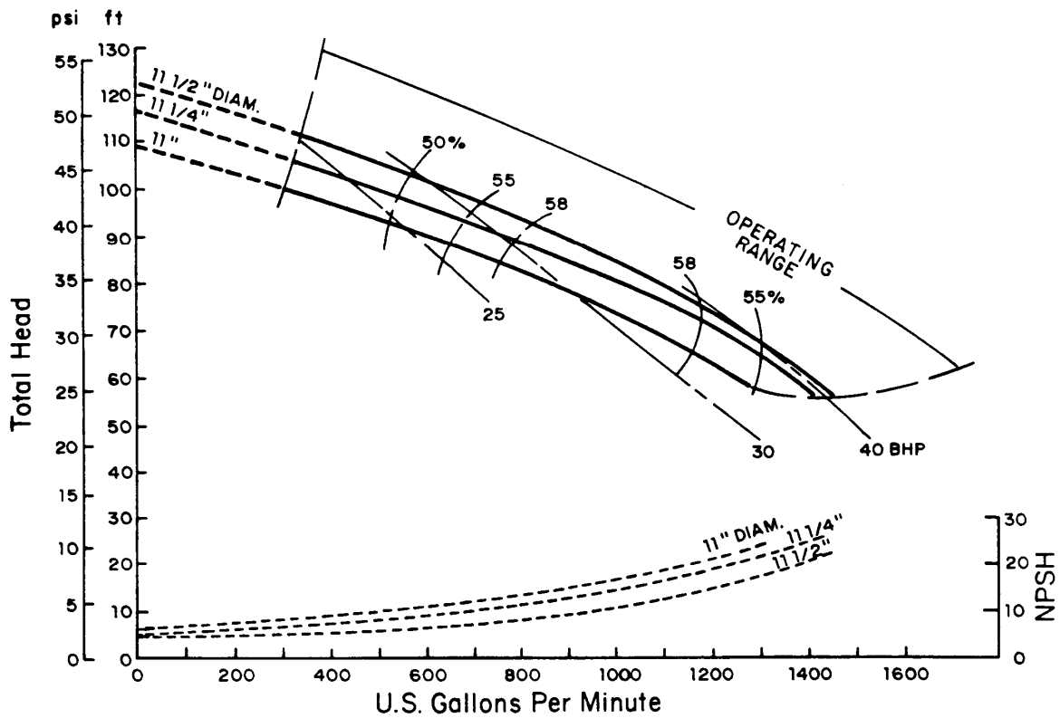
Figure 5: Typical Manufacturer's Pump Curve (Adapted from G-R Pump Curve)
