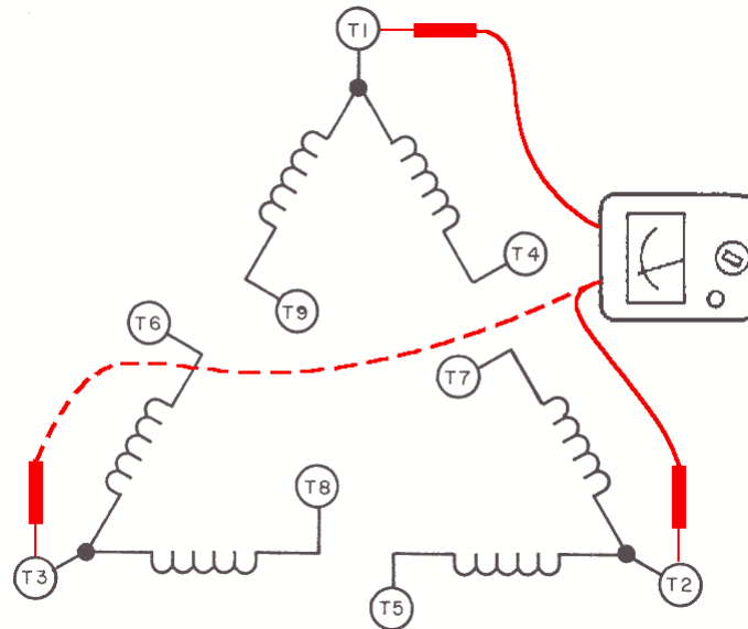
Figure 22: Motor Coil to Coil Insulation Check
