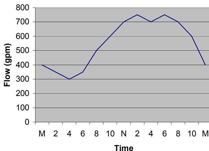
Figure 11: Typical Diurnal Flow Variations
