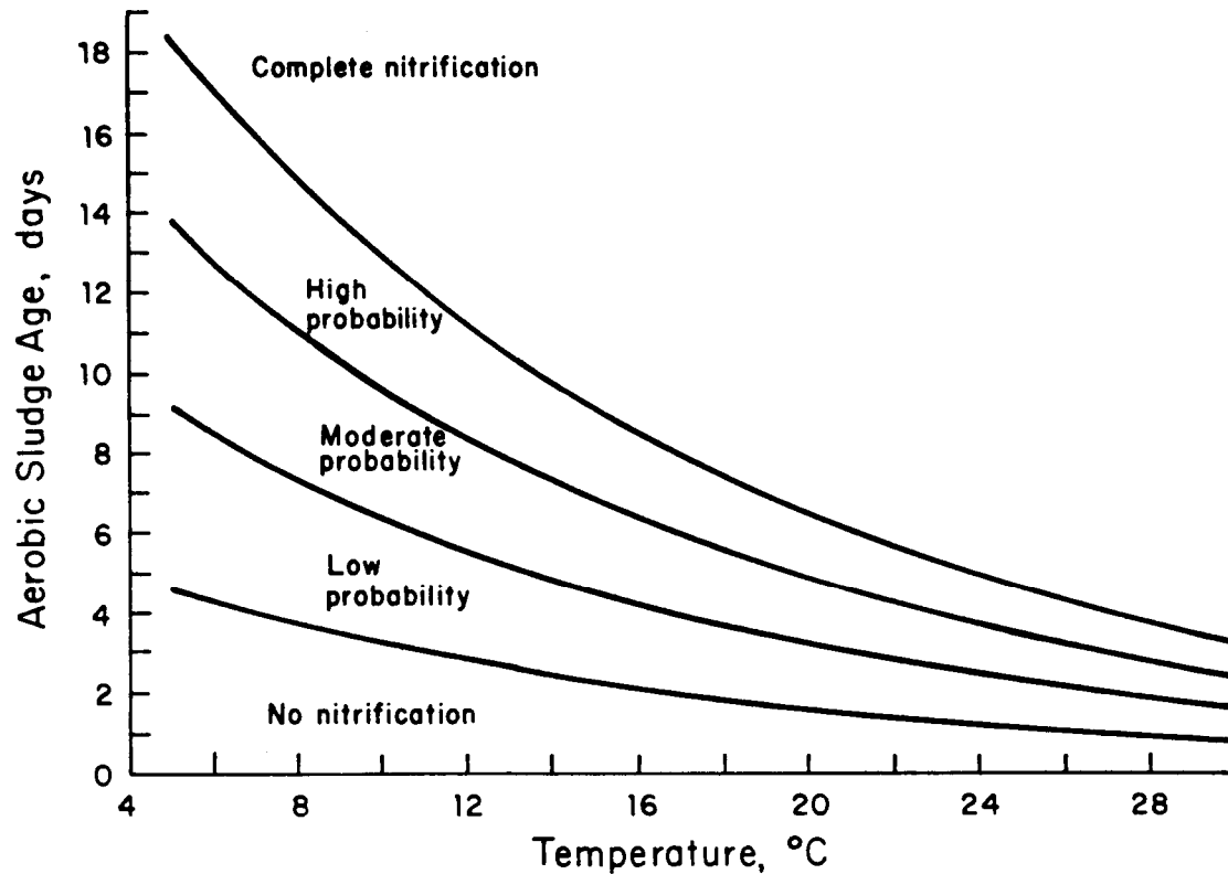
Figure 14: Nitrification Potential in Activated Sludge
