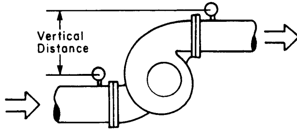
Figure 2: Head Correction for Pressure Gauge Location
