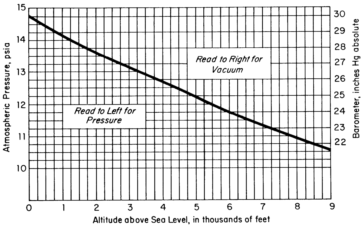
Figure 15: Atmospheric Pressure at Various Altitudes (EPA 1984)
