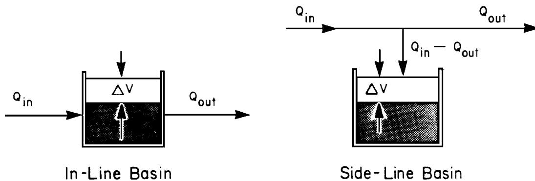
Figure 12: Simple Flow Balance Schematics (EPA 1979)
