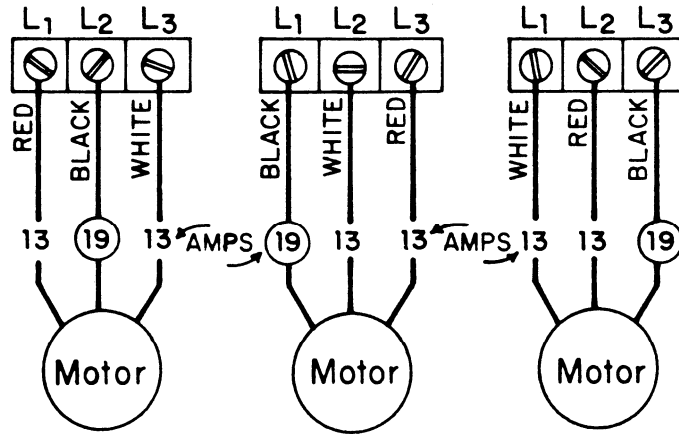
Figure 19: Unbalance Caused by Load (Adapted from FLYGT)
