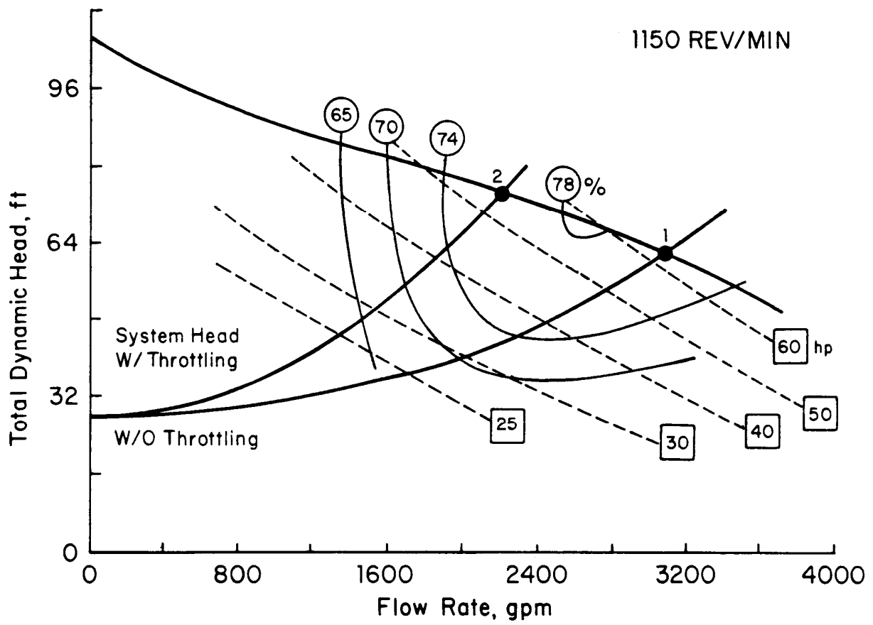
Figure 6: Pump Throttling (Adapted from GIT, 1981)
