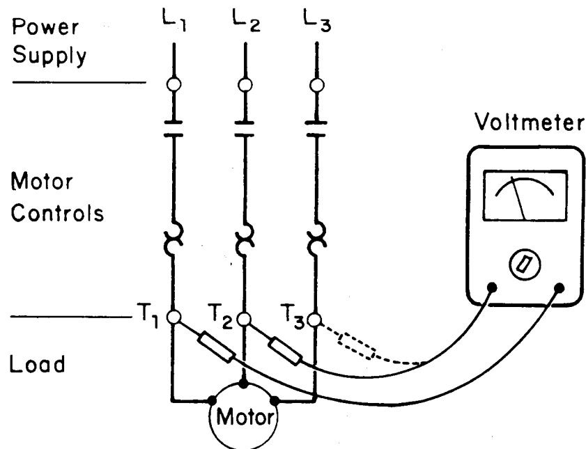
Figure 17: Checking 3-Phase Motor Voltage (Adapted from FLYGT)
