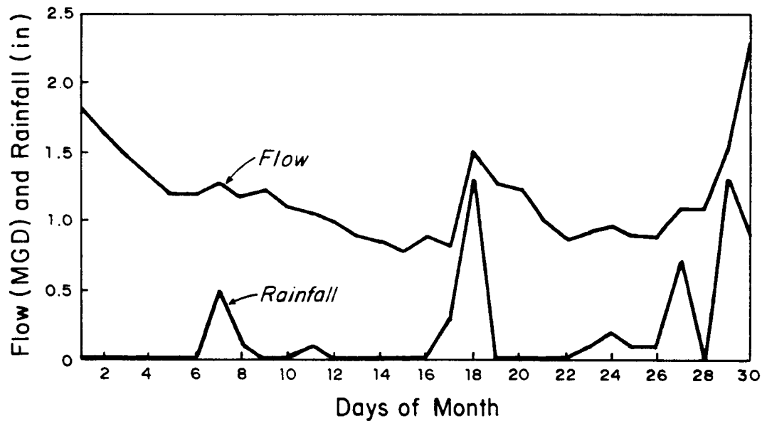
Figure 10: Wet Weather Flow and Rainfall
