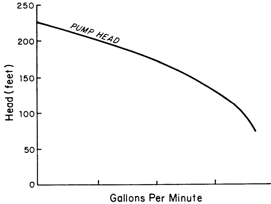
Figure 4: Basic Pump Curve (TREEO, 1986)
