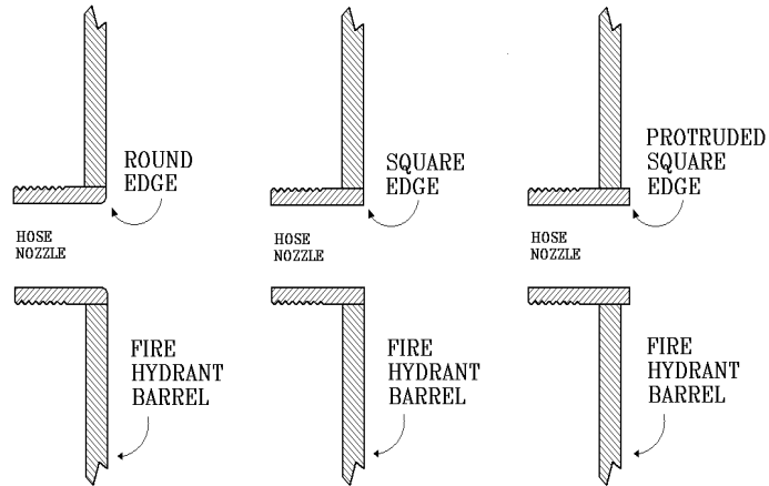
Figure 8: Value for nozzle coefficient
