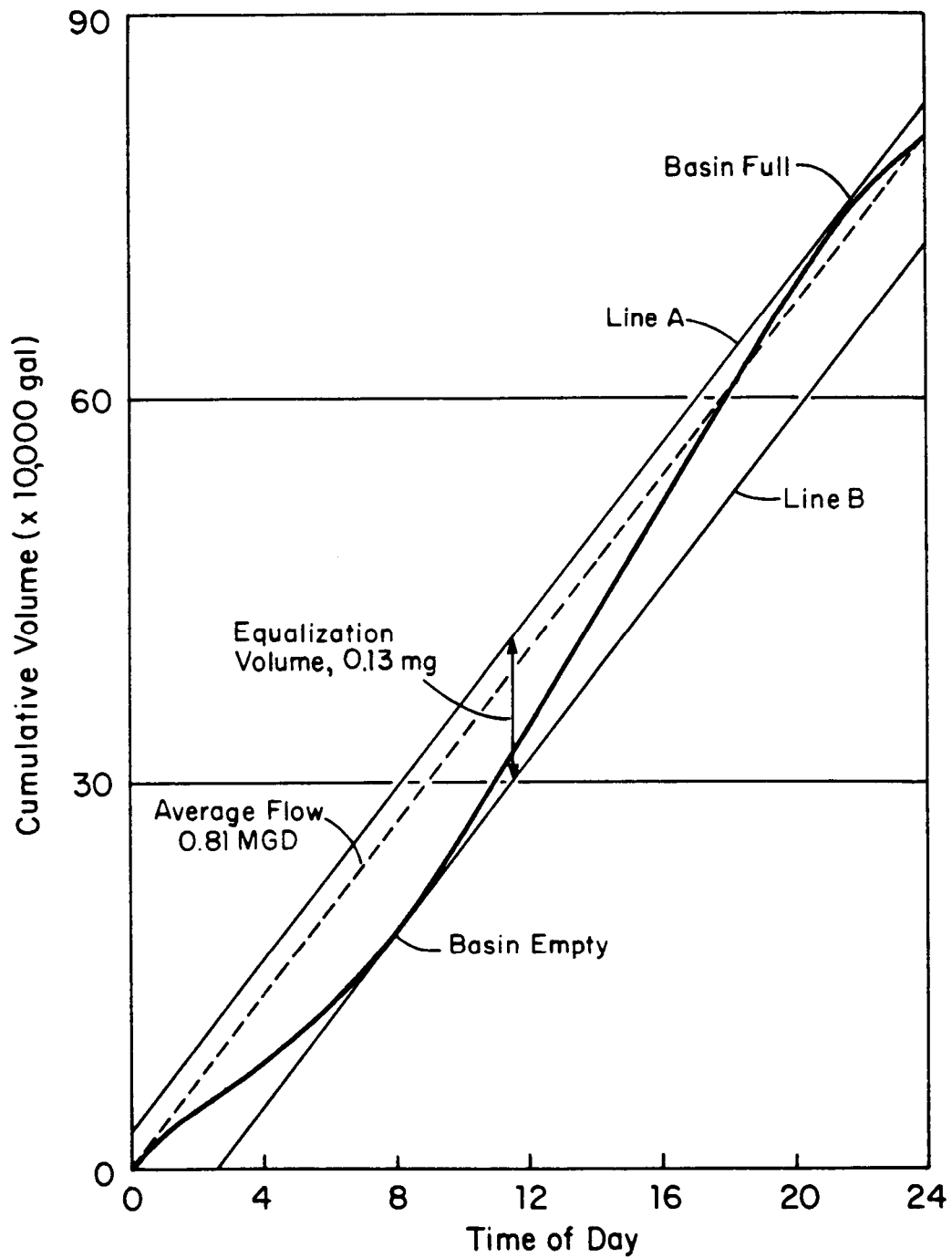
Figure 13: Hydrograph of Figure 7 Diurnal Flow Data
