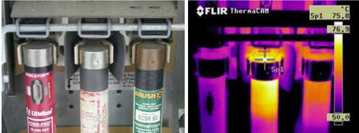
Figure 26: Overheating fuse (Courtesy of FLIR Systems, Inc., N. Billerica, MA
