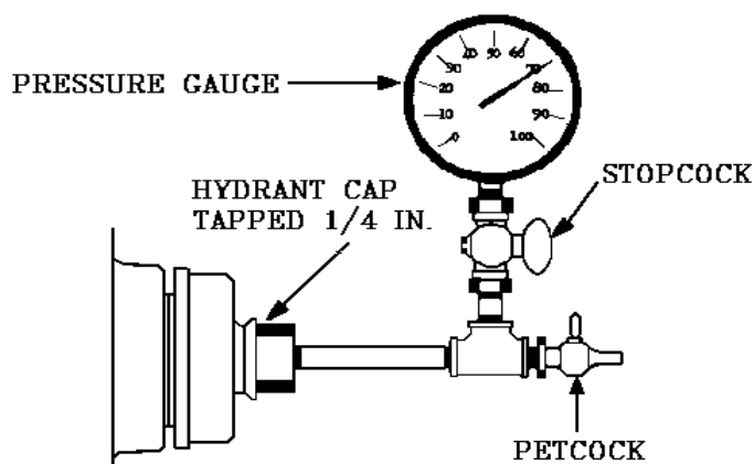
Figure 7: Hydrant cap gauge (After AWWA 1986(1))
