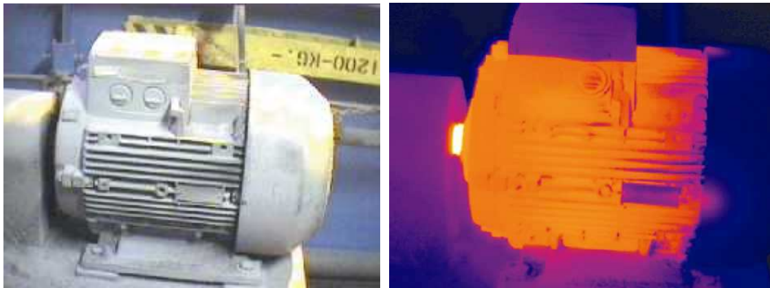
Figure 25: Bad windings ( Courtesy of FLIR Systems, Inc., N. Billerica, MA)
