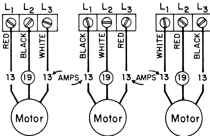
Figure 20: Unbalance Caused on Supply Side of Controls (Adapted from FLYGT)
