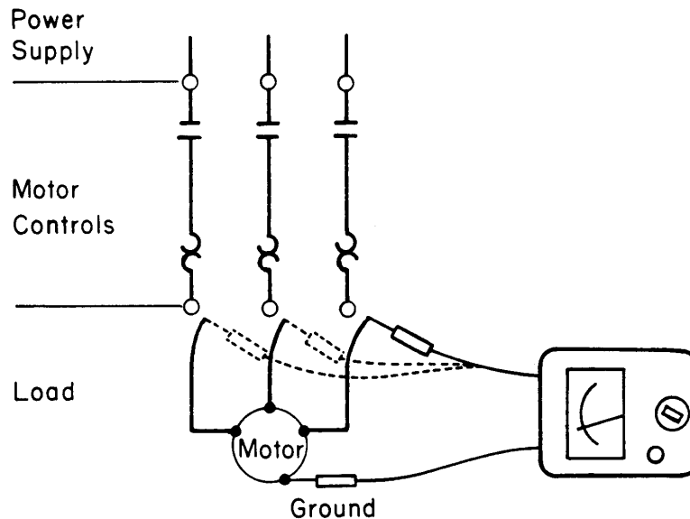
Figure 21: Checking Primary Insulation (Adapted from FLYGT)
