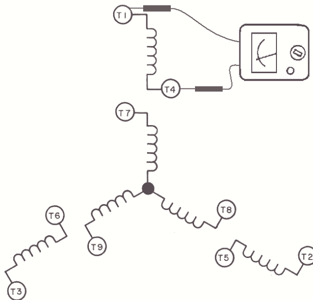
Figure 23: Testing for coil open circuits
