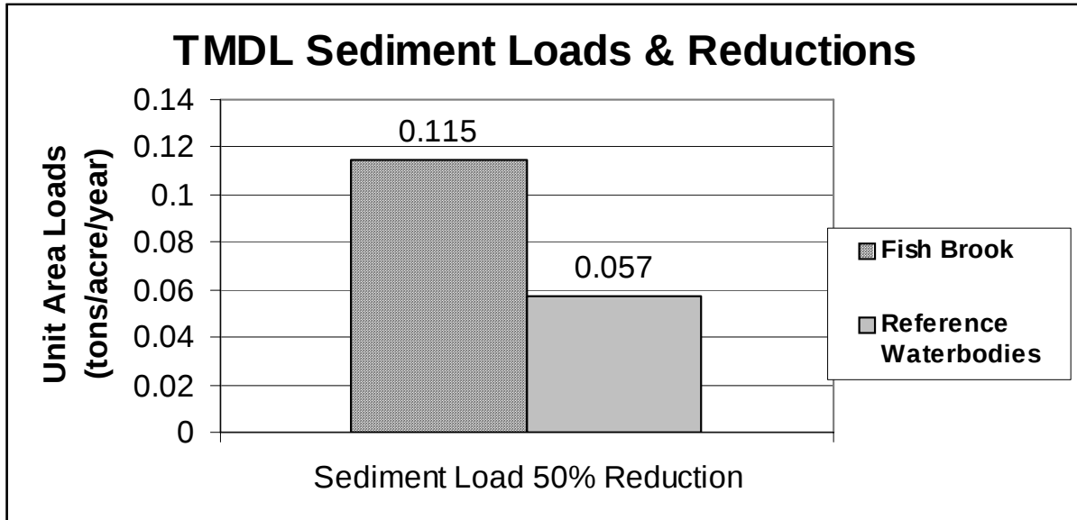
Figure 9. Sediment load estimates compared between the watersheds and reductions needed to achieve compliance with Maine's Class B water quality standards in the impaired stream segment.
