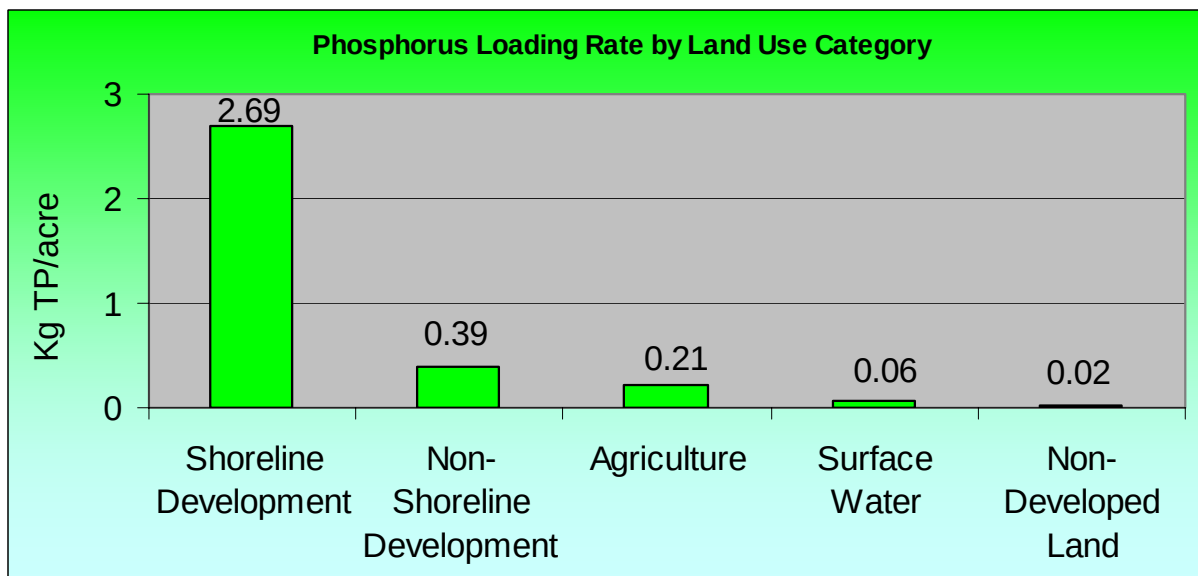
Figure 2b TP Loading Rates by Land Use Class
