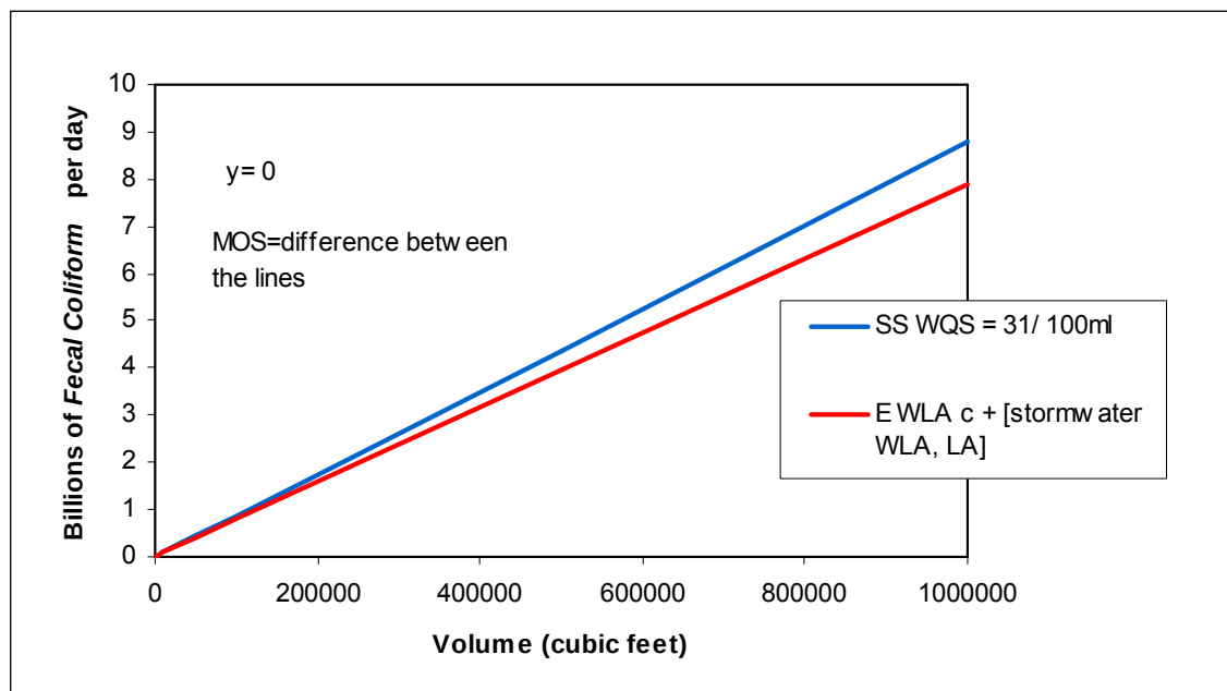
Figure 5. Marine and Estuarine Mass per Unit Time TMDL based on 90 th Percentile Water Quality Standard.
