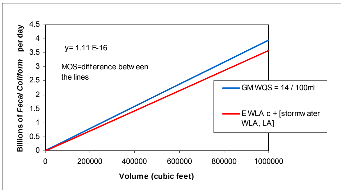
Figure 6. Marine and Estuarine Mass per Unit Time TMDL based on Geometric Mean Water Quality Standard.
