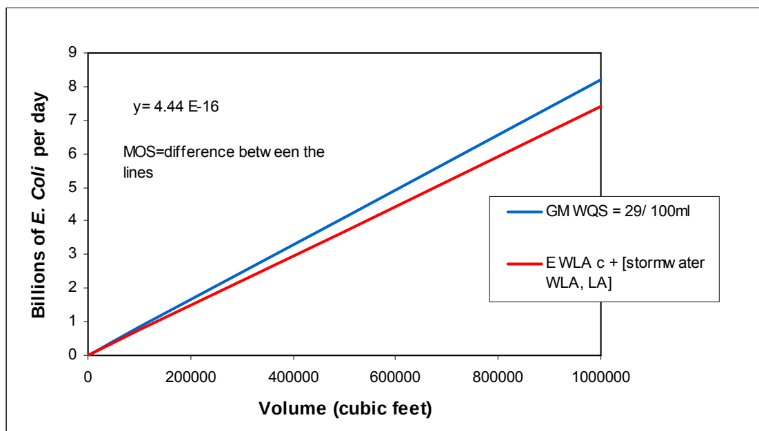
Figure 4. Lake and Pond Mass per Unit Time TMDL based on Geometric Mean Water Quality Standard.
