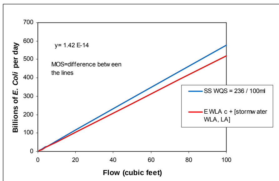
Figure 1. River and Stream Mass per Unit Time TMDL based on Single Sample Water Quality Standard.
