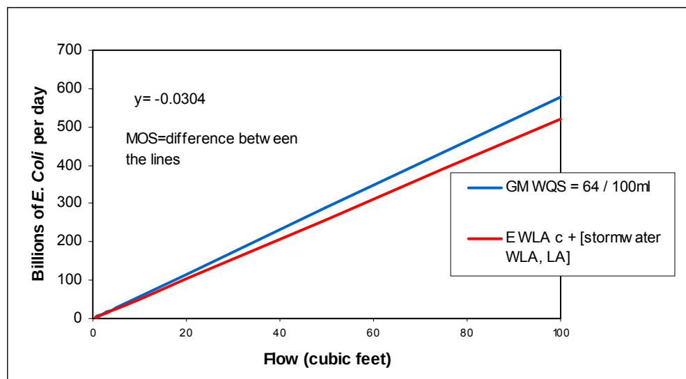
Figure 2. River and Stream Mass per Unit Time TMDL based on Geometric Mean Water Quality Standard.
