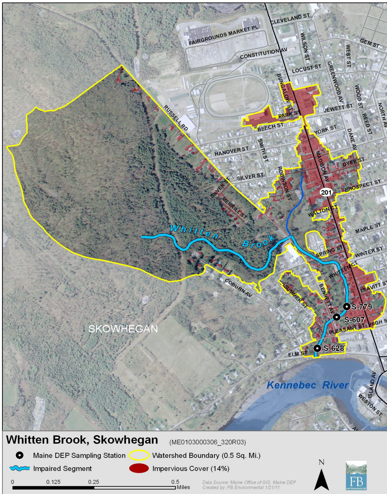
Figure 1: Map of Whitten Brook watershed impervious cover.
