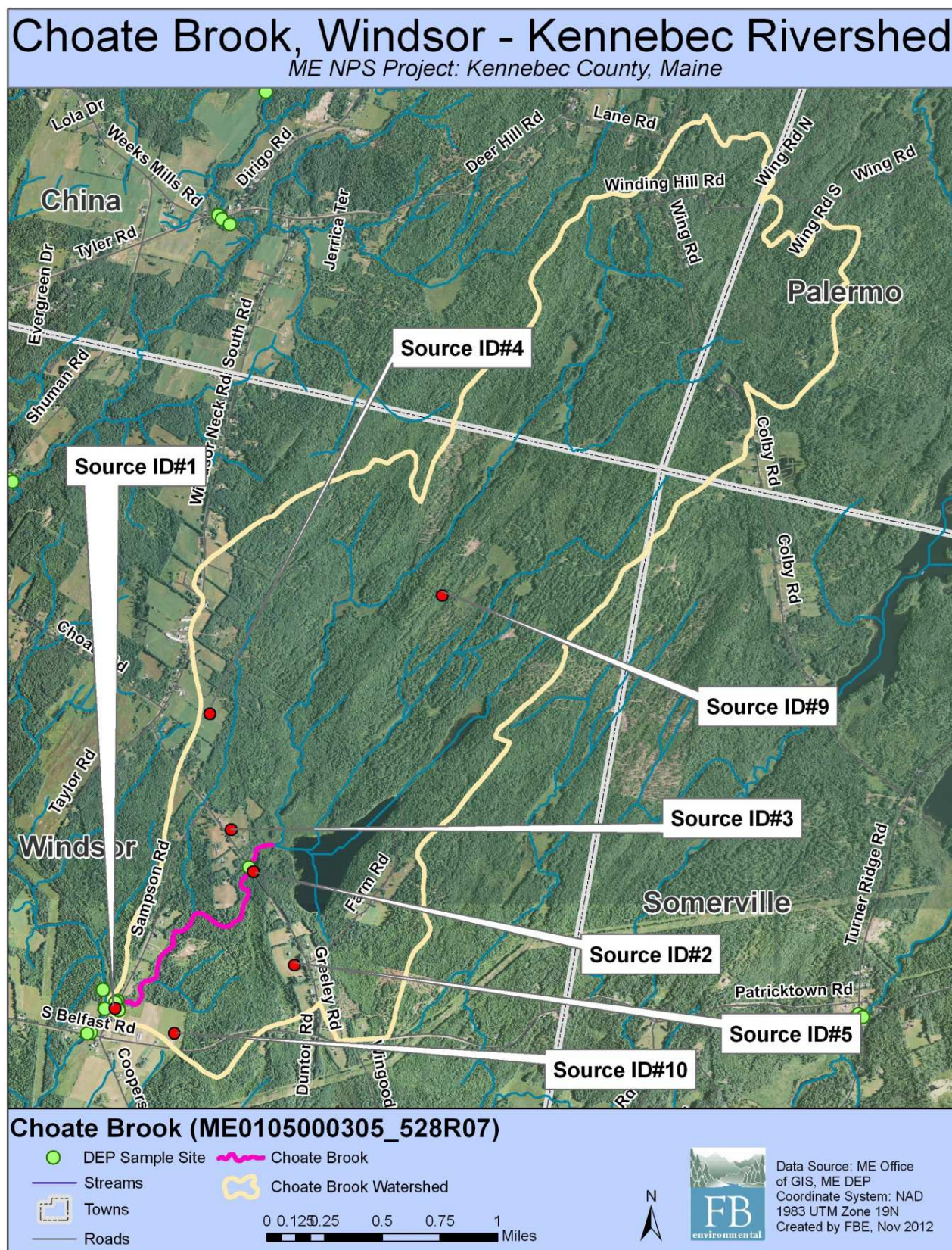
Figure 3: Aerial Photo of Source ID Locations in the Choate Brook Watershed
