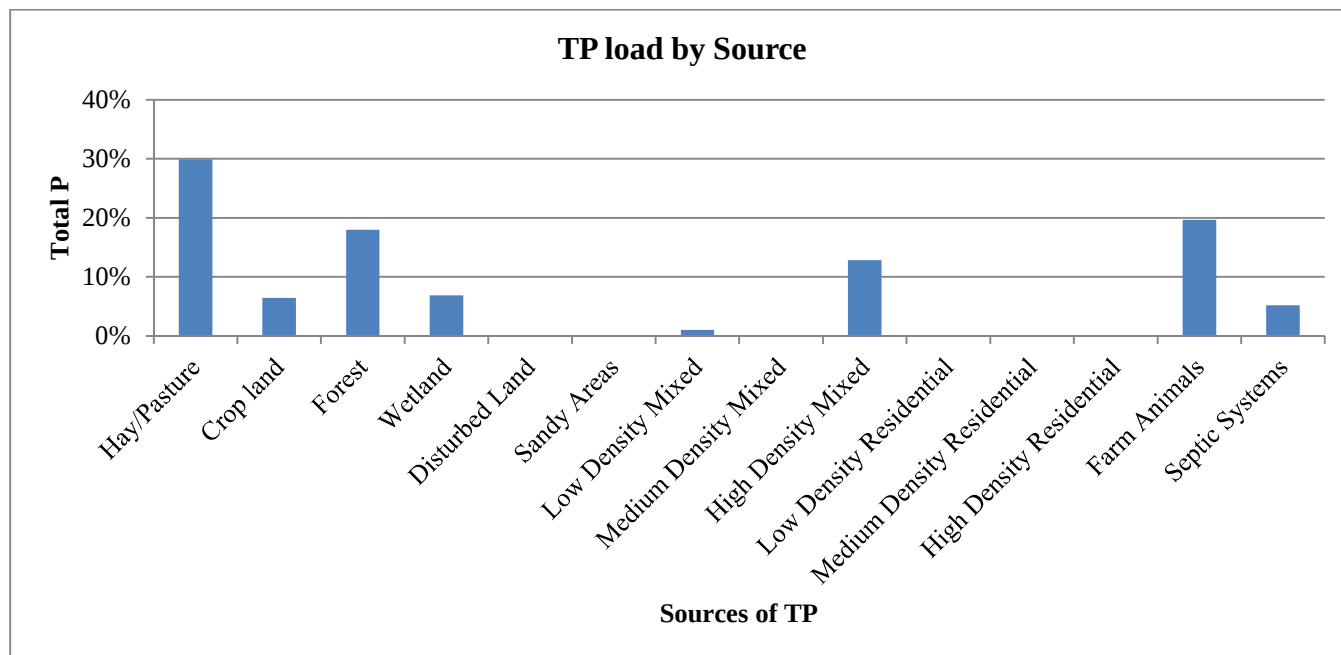
Figure 7: Total Phosphorus Loads by Source in the Choate Brook Watershed
