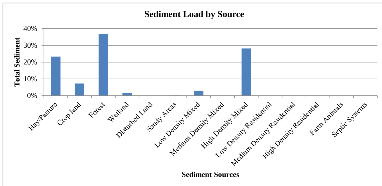
Figure 5: Total Sediment Loads by Source in the Choate Brook Watershed
