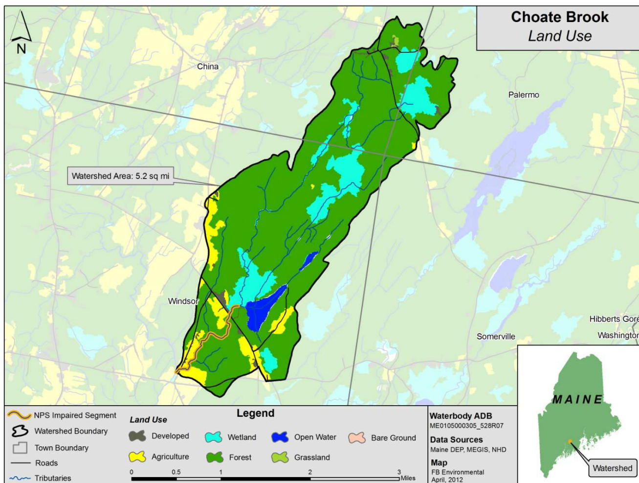
Figure 1: Land Use in the Choate Brook Watershed
