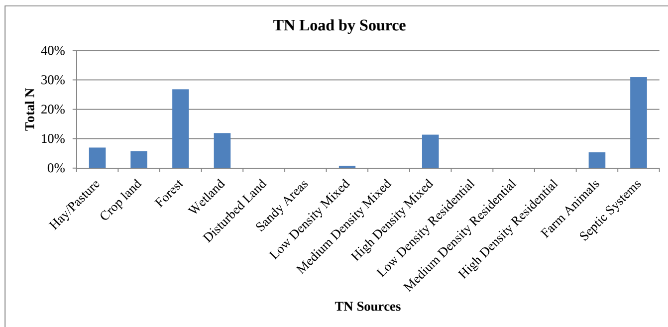
Figure 6: Total Nitrogen Loads by Source in the Choate Brook Watershed
