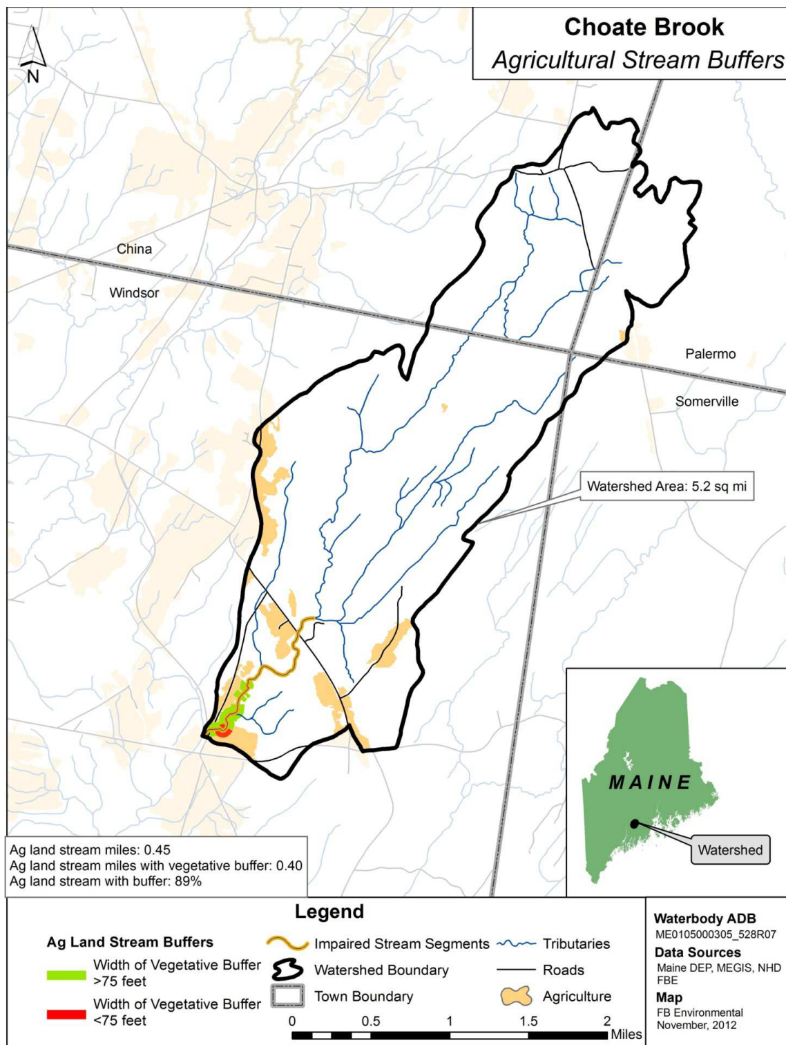
Figure 4: Agricultural Stream Buffer in the Choate Brook Watershed
