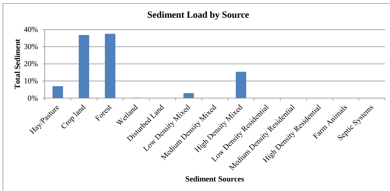
Figure 5: Total Sediment Loads by Source in the Carlton Brook Watershed
