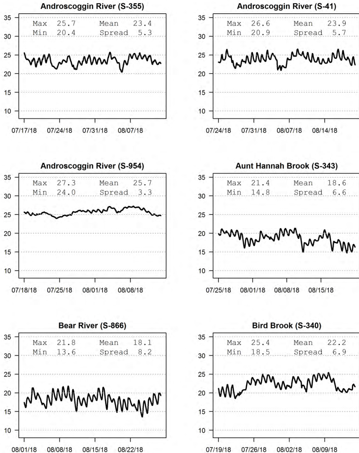
Figure 3.1.1b 2018 In-Stream Continuous Temperature Data
