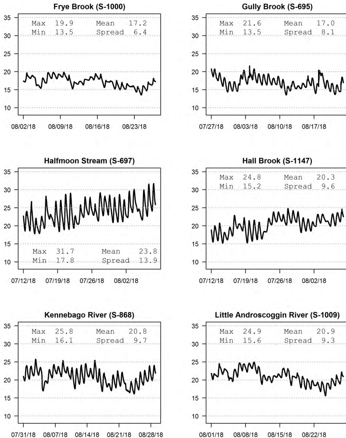
Figure 3.1.1b 2018 In-Stream Continuous Temperature Data (continued)
