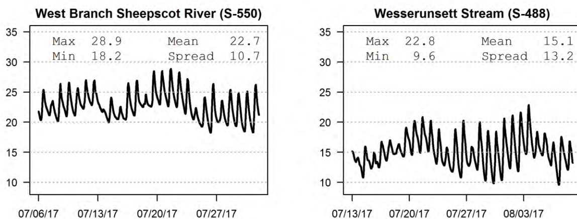
Figure 3.1.1a 2017 In-Stream Continuous Temperature Data (continued)
