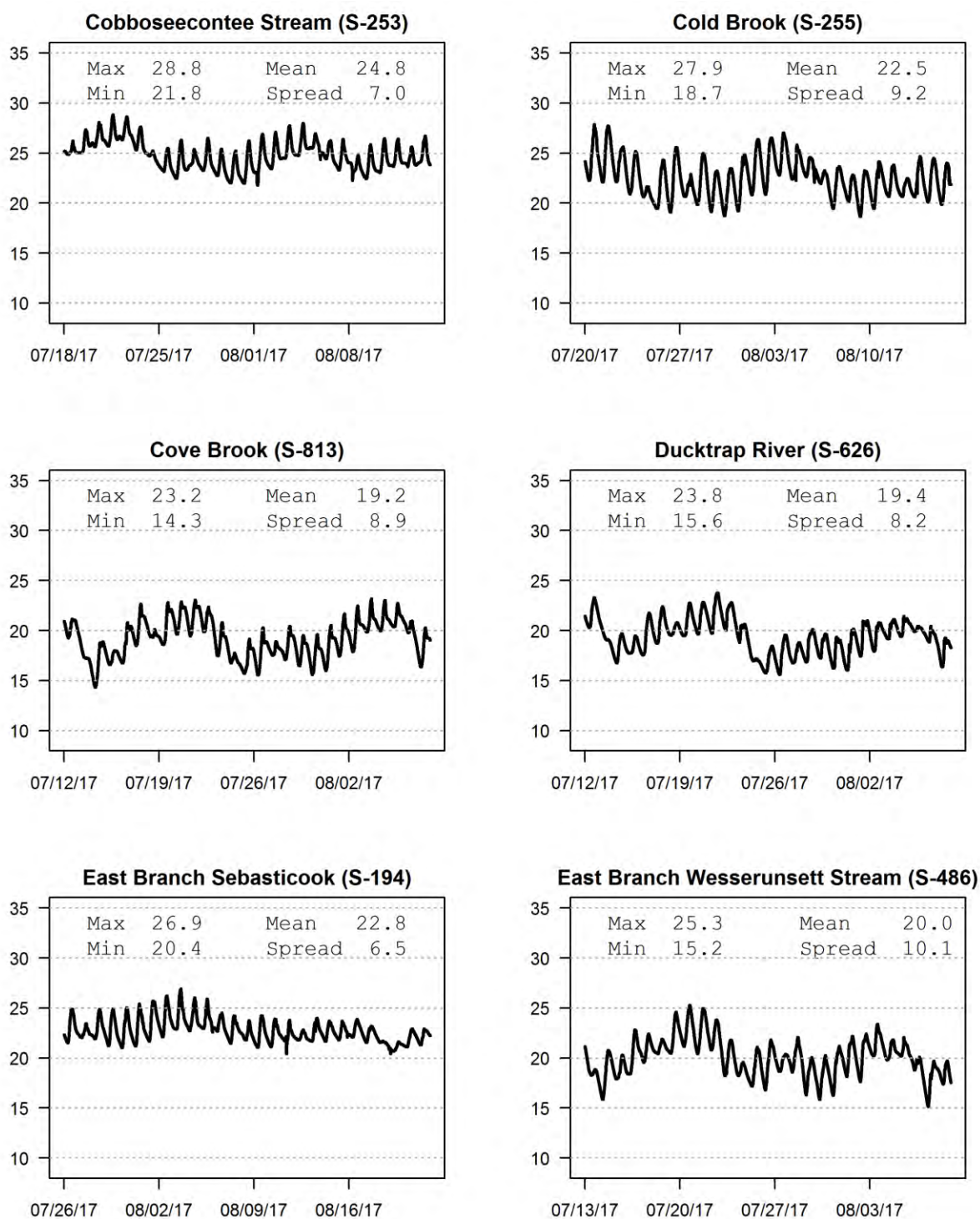
Figure 3.1.1a 2017 In-Stream Continuous Temperature Data (continued)
