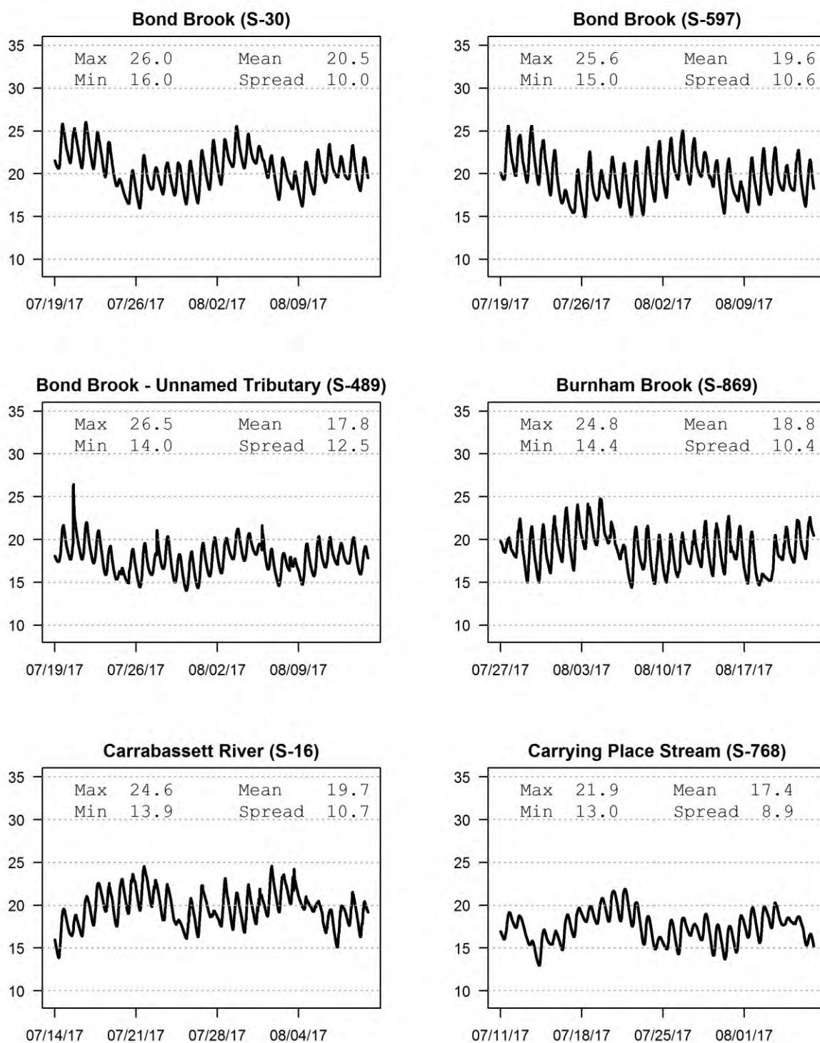
Figure 3.1.1a 2017 In-Stream Continuous Temperature Data
