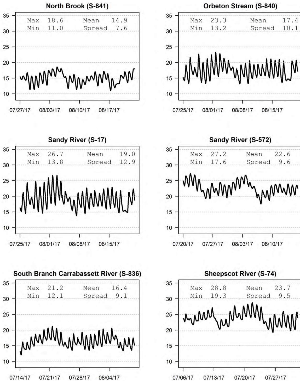
Figure 3.1.1a 2017 In-Stream Continuous Temperature Data (continued)
