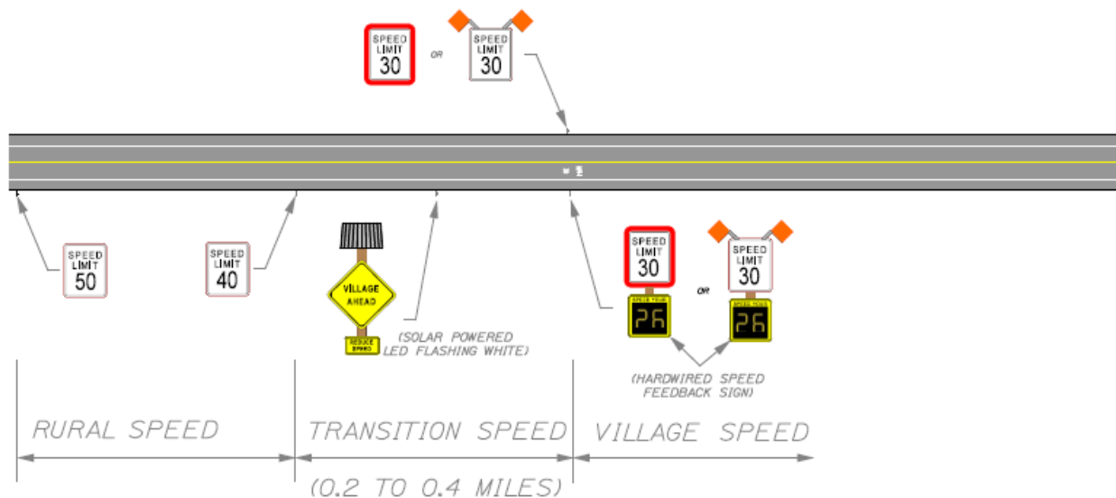
Fig.2 - Dynamic Signs
