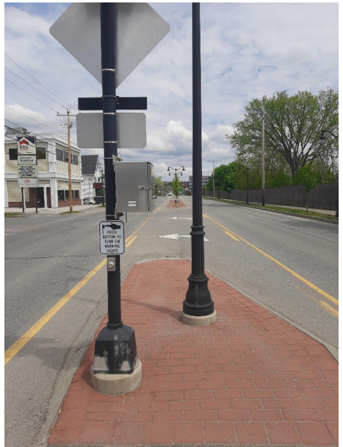
Bangor Main St Median Island- View From Island Showing Lighting Standards
