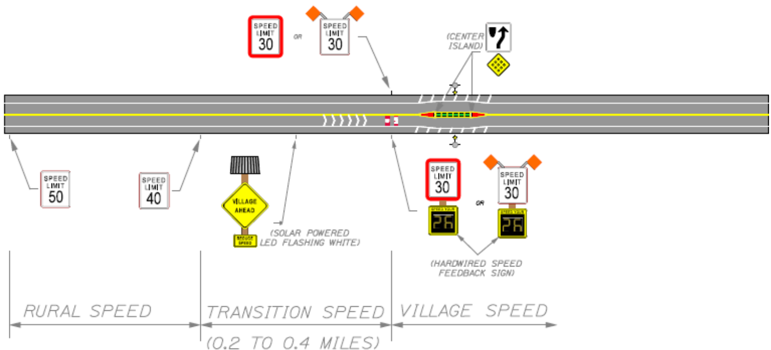
Fig.3 - Center Island
