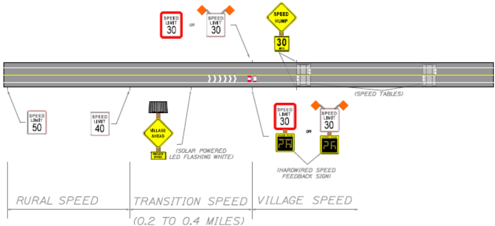
Fig.5 - Speed Tables
