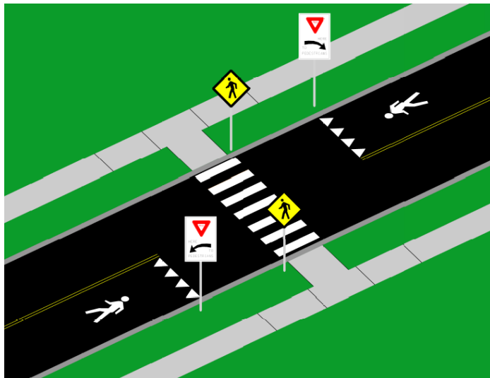
Figure 10 – Crosswalks with Yield Bars and Enhanced Signage
