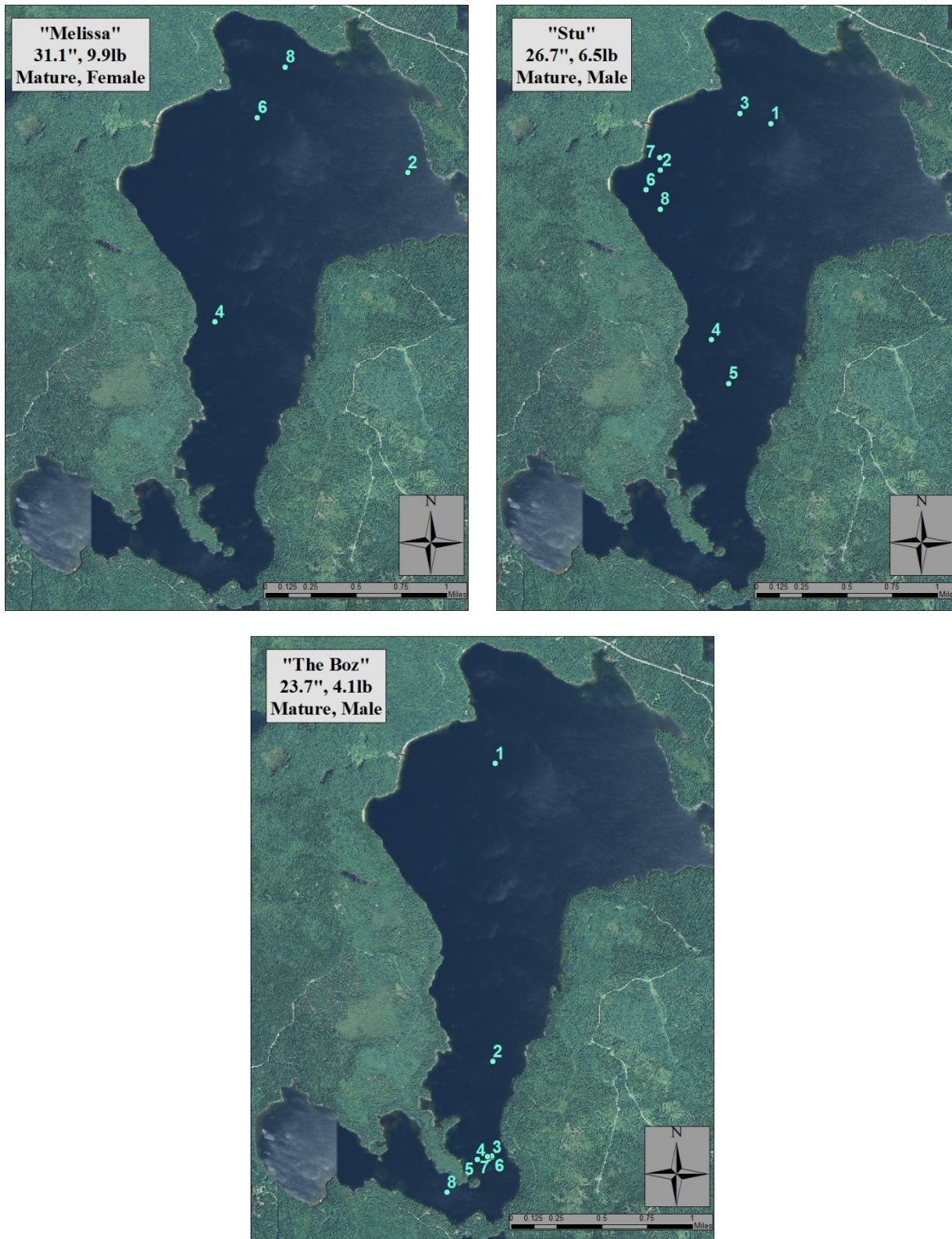
Figure 5c: Individual fish locations labeled by tracking event
